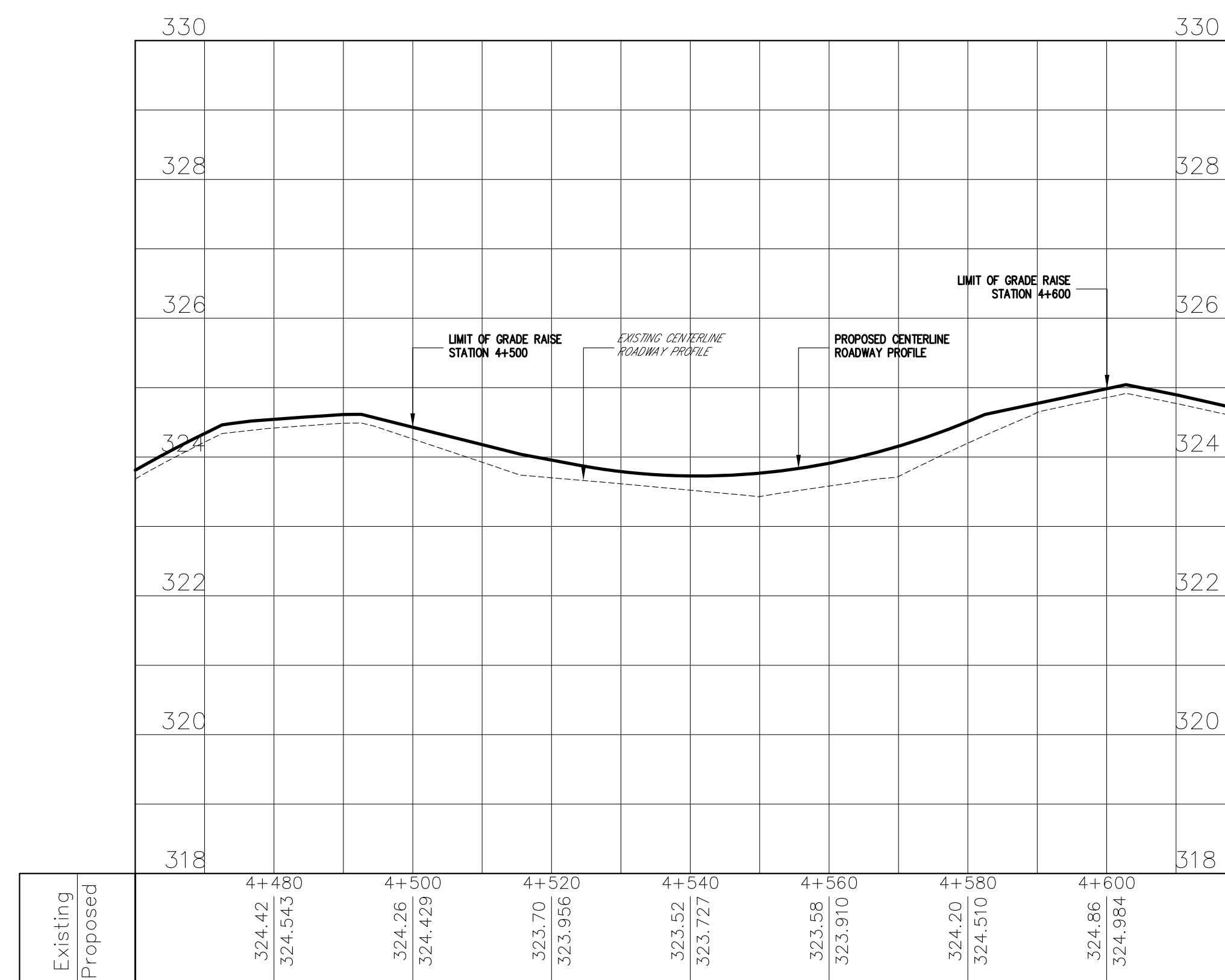
GRADE RAISE #3
