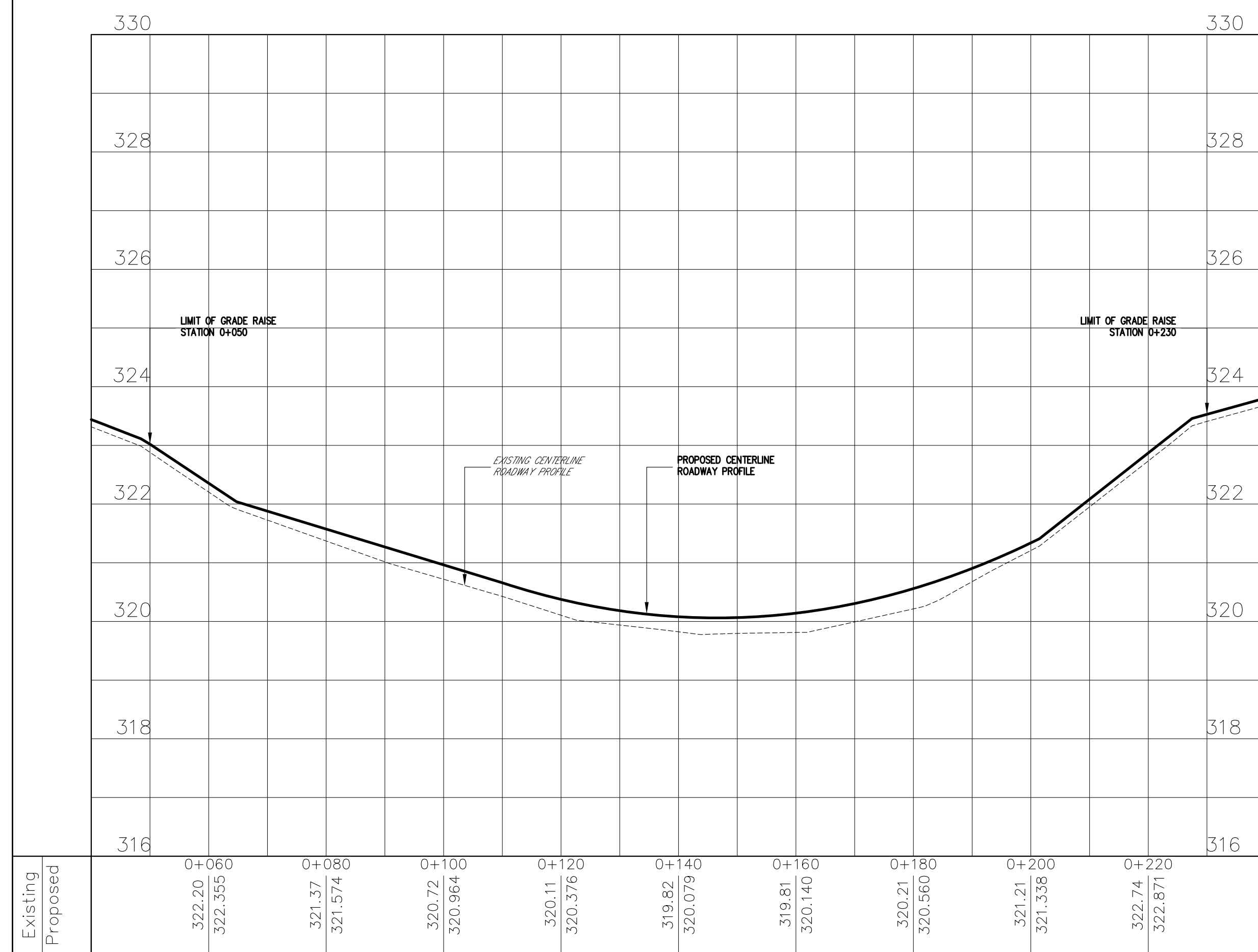
GRADE RAISE #1
