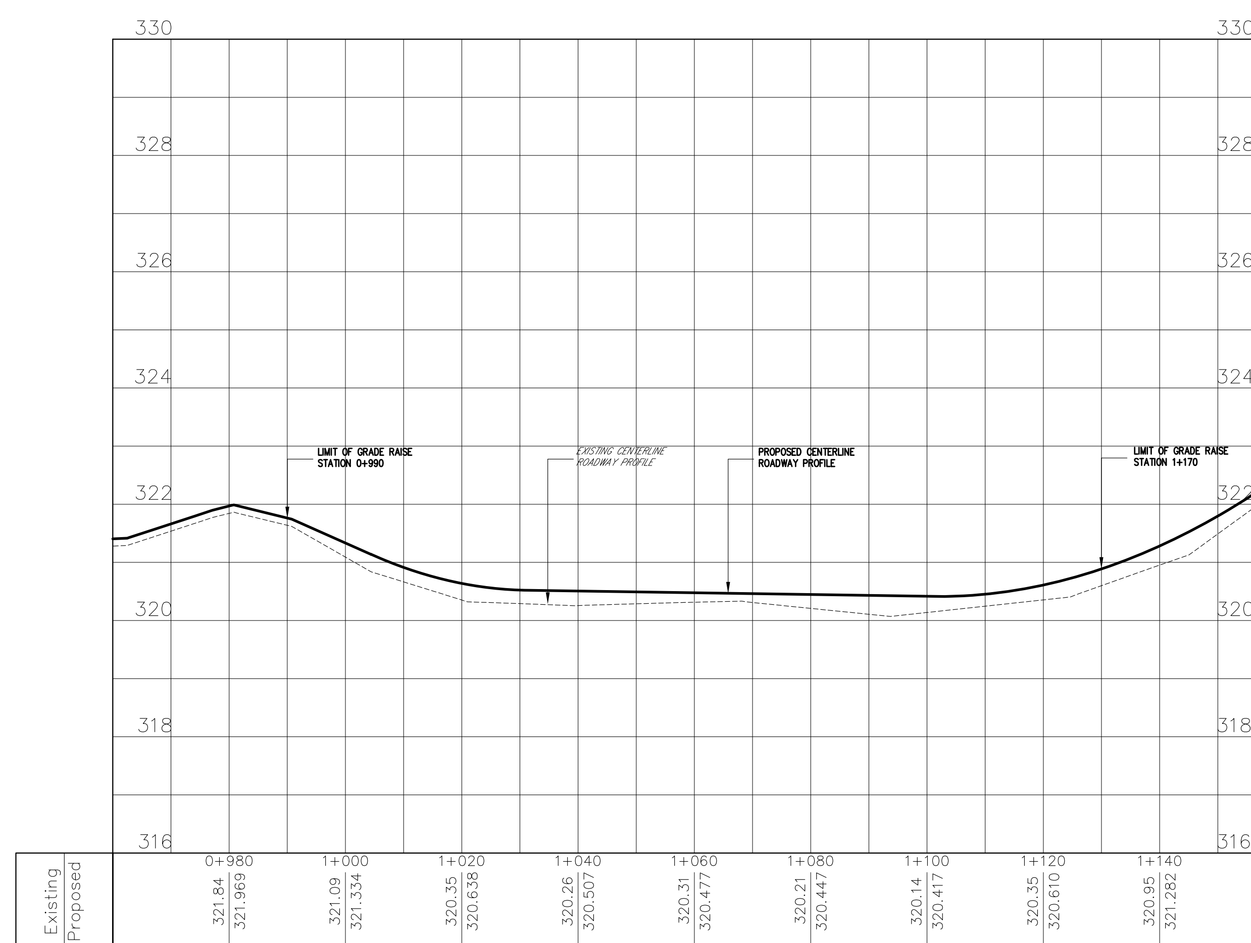
GRADE RAISE #2
